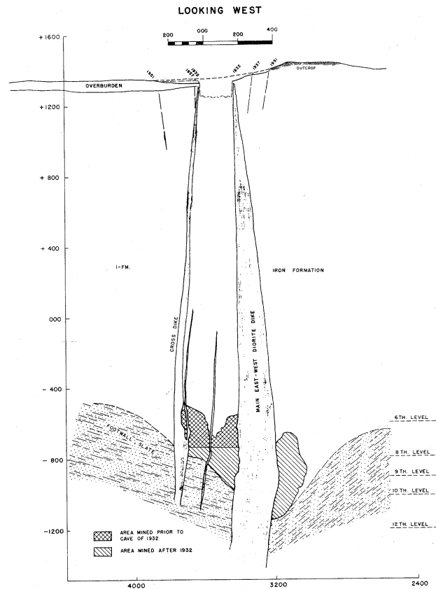
Figure 7 Schematic of surface subsidence observed at the Athens Mine (Boyum, 1961)
