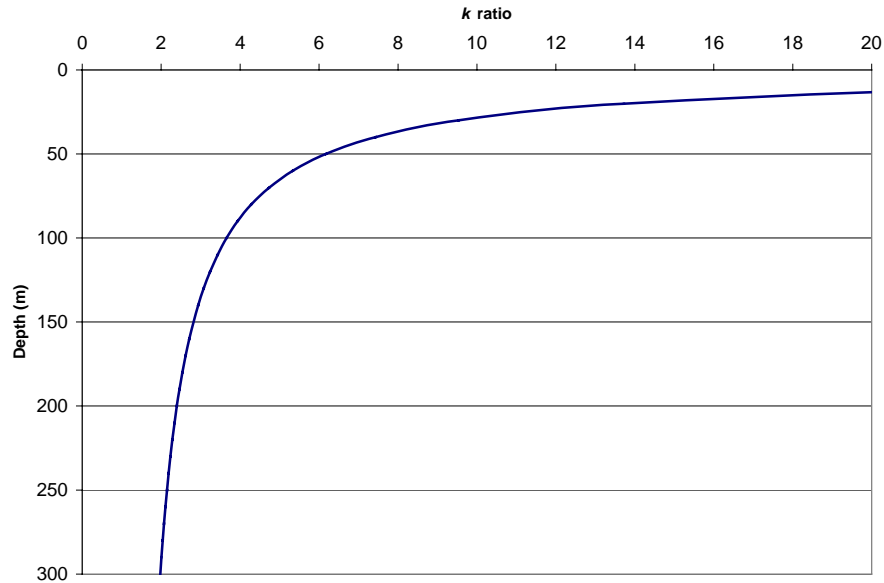
Figure 5 Variation of k ratio with depth based upon Herget's (1988) equation
