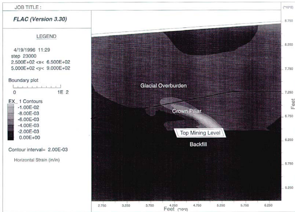
Figure 8 Location of excessive rock mass strain within Crandon crown pillar (Hardy et al., 1999)
