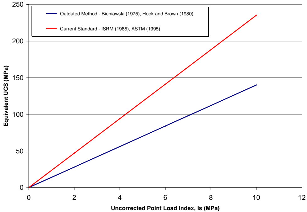
Figure 3 Comparison between equivalent UCS obtained using outdated method and the current ISRM and ASTM methods assuming the default conversion factor of 24
