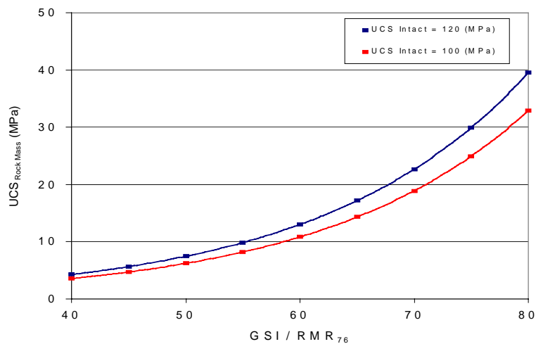
Figure 4 Increase in UCS_{rock\ mass} with increasing GSI or RMR 76
