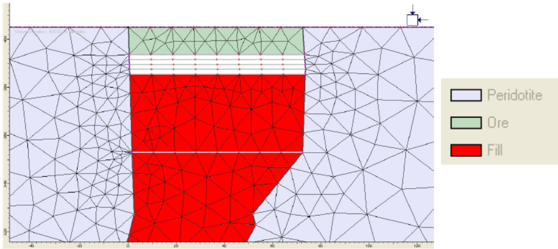
Figure 6 Phase 2 model geometry and finite element mesh (Golder, 2006c)
