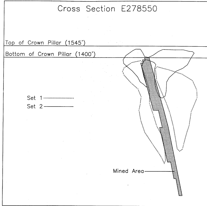
Figure 9 Contours of factor of safety = 1 for predominant joint sets (width of orebody = 100 ft) (Hardy et al., 1999)
